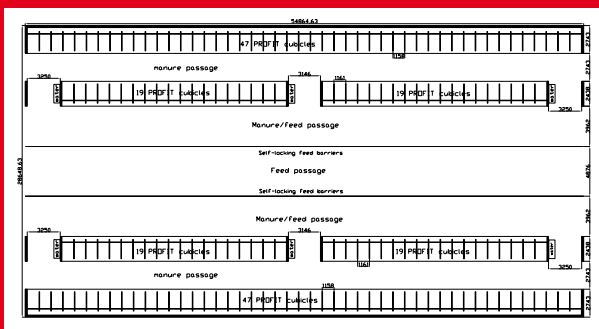
Computer aided illustration of a typical cubicle layout
